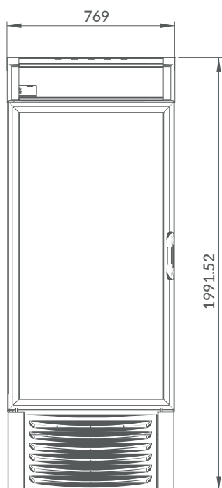
Vista frontal
